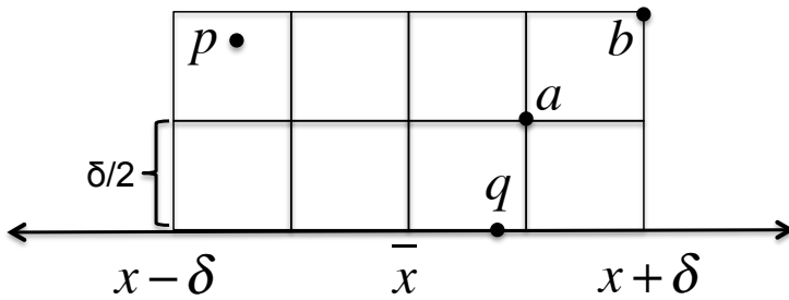
Figure 3.7: Proof of Lemma 3.3(b). The points p and q inhabit two of these eight boxes, and there is at most one point in each box.
